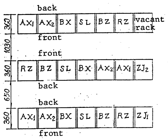
Figure 3. 600-Line Arrangement
