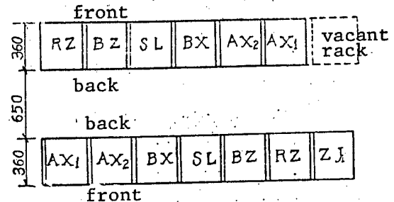
Figure 2. 400-Line Arrangement
