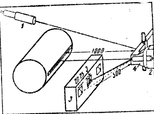
Fig. 1. Diagram of the optical part of the APZO 1 - additional collimator; 2 - galvanometer; 3 - photoelement; 4 - coarse-tuning marker.
