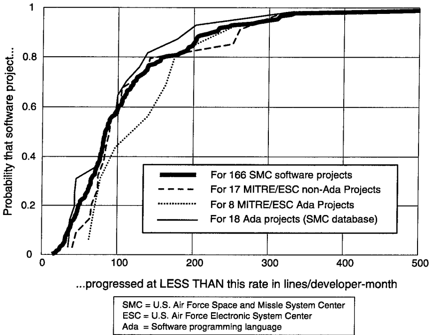
FIGURE 4-1 Historical software coding rates. Source: The Aerospace Corporation, 1998.
