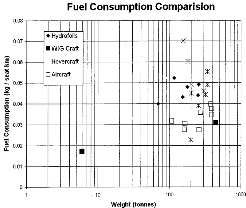
Figure 15 Fuel Consumption [24]
