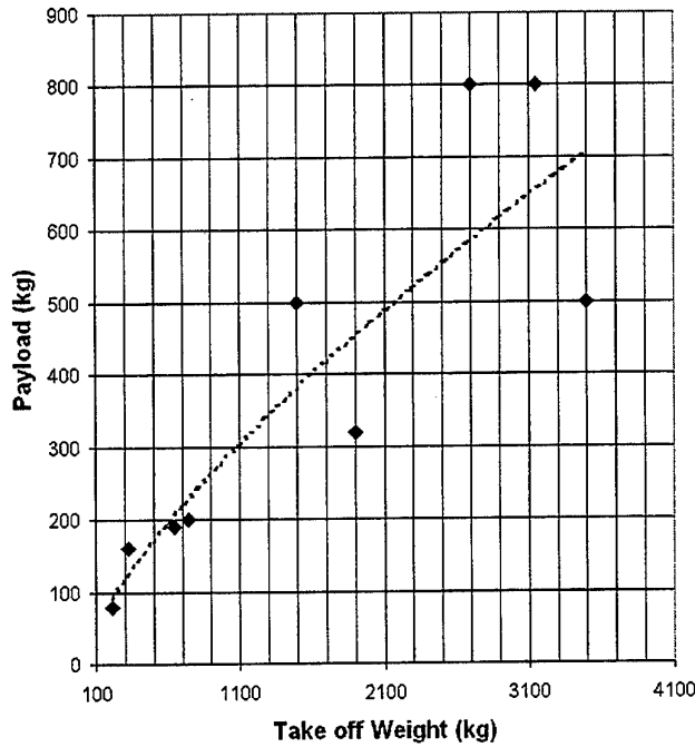
Figure 18 Payload for Various Size WIG Craft.
