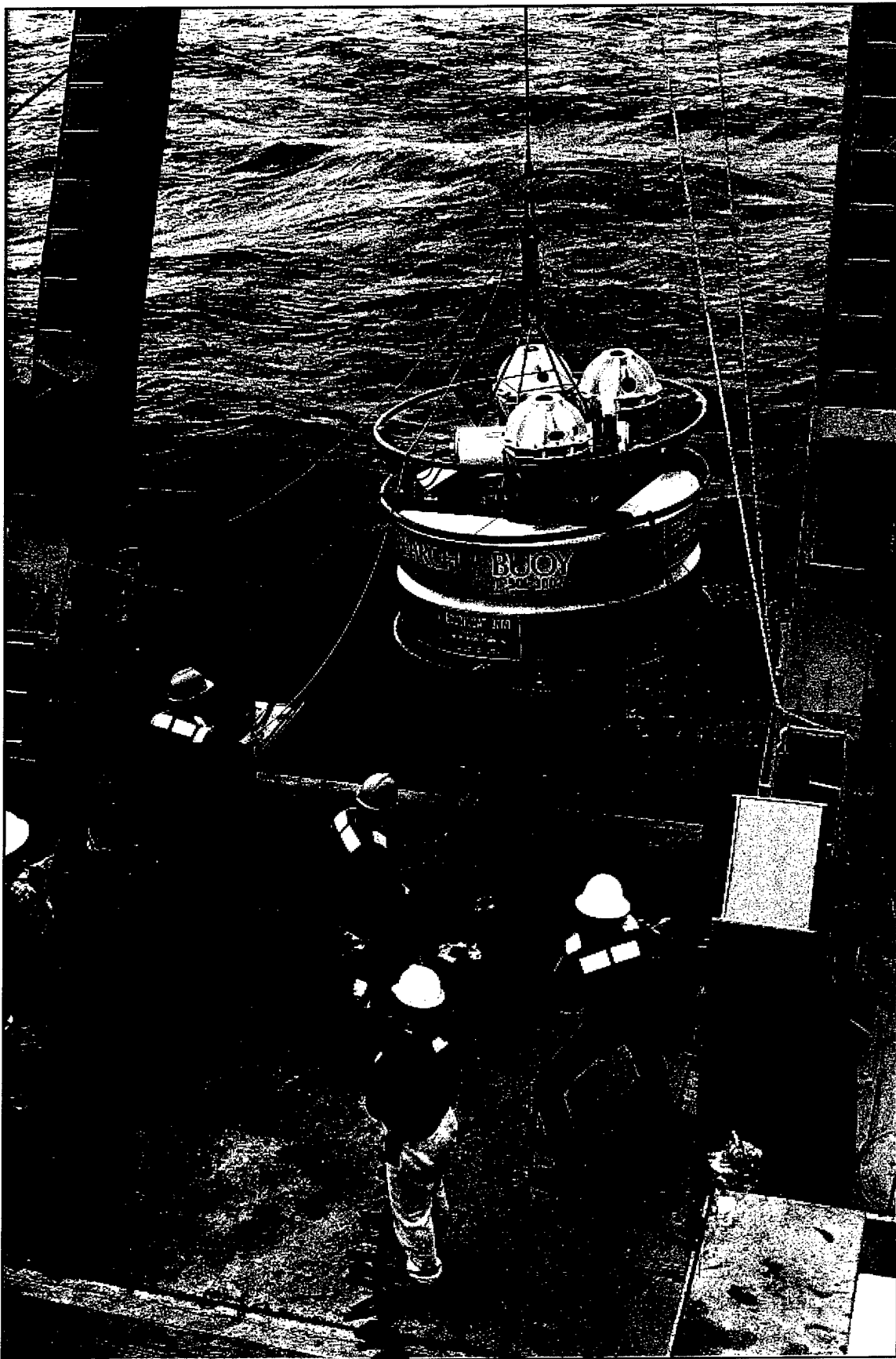
Subsurface float deployment from the R/V Melville during July, 1998 for the North Pacific Acoustic Laboratory (NPAL) experiment. The subsurface float can carry up to four pop-up buoys for mid-experiment data retrieval.
