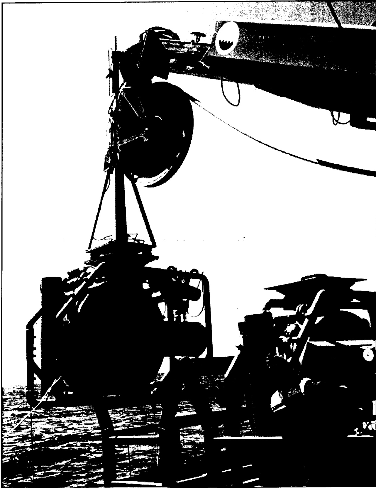
Deployment of an HLF-6A acoustic source (28 Hz and 84 Hz) near Pioneer Seamount off central California for the Dual-Frequency Test in July, 1996.
