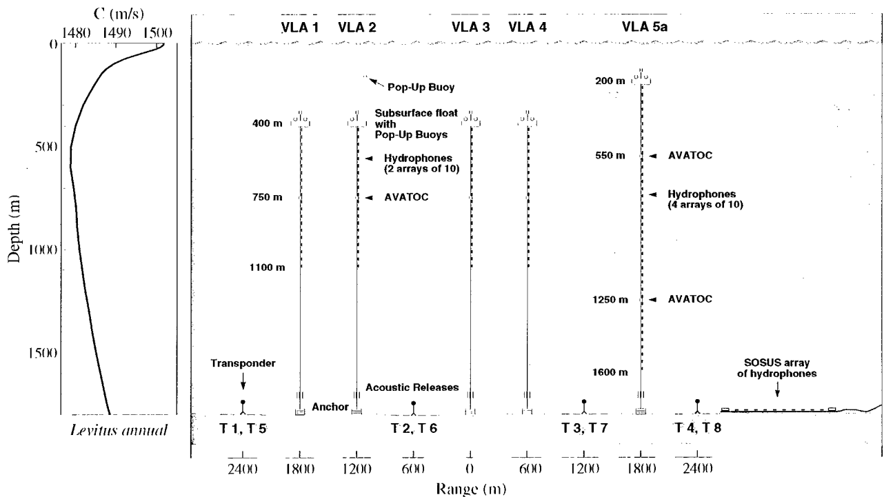
Vertical Line Array (VLA) receivers deployed off Pt. Sur, California, during July, 1998 for the North Pacific Acoustic Laboratory (NPAL) experiment. The VLAs were deployed transverse to the acoustic path from the ATOC source installed north of Kauai.
