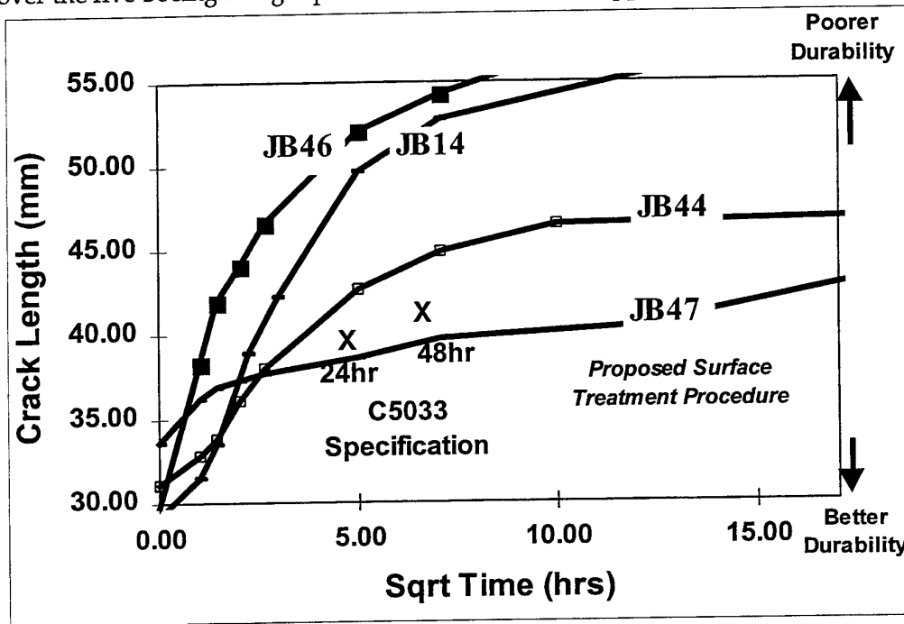
Figure 2: Boeing wedge durability tests trial surface treatments for the Aluminium 7075 and FM73 system. The JB reference refers to surface treatments given in Table 2.
