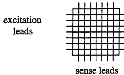
Figure 1. Grid Showing 64 Points of Intersection for Excitation and Sense Leads.
