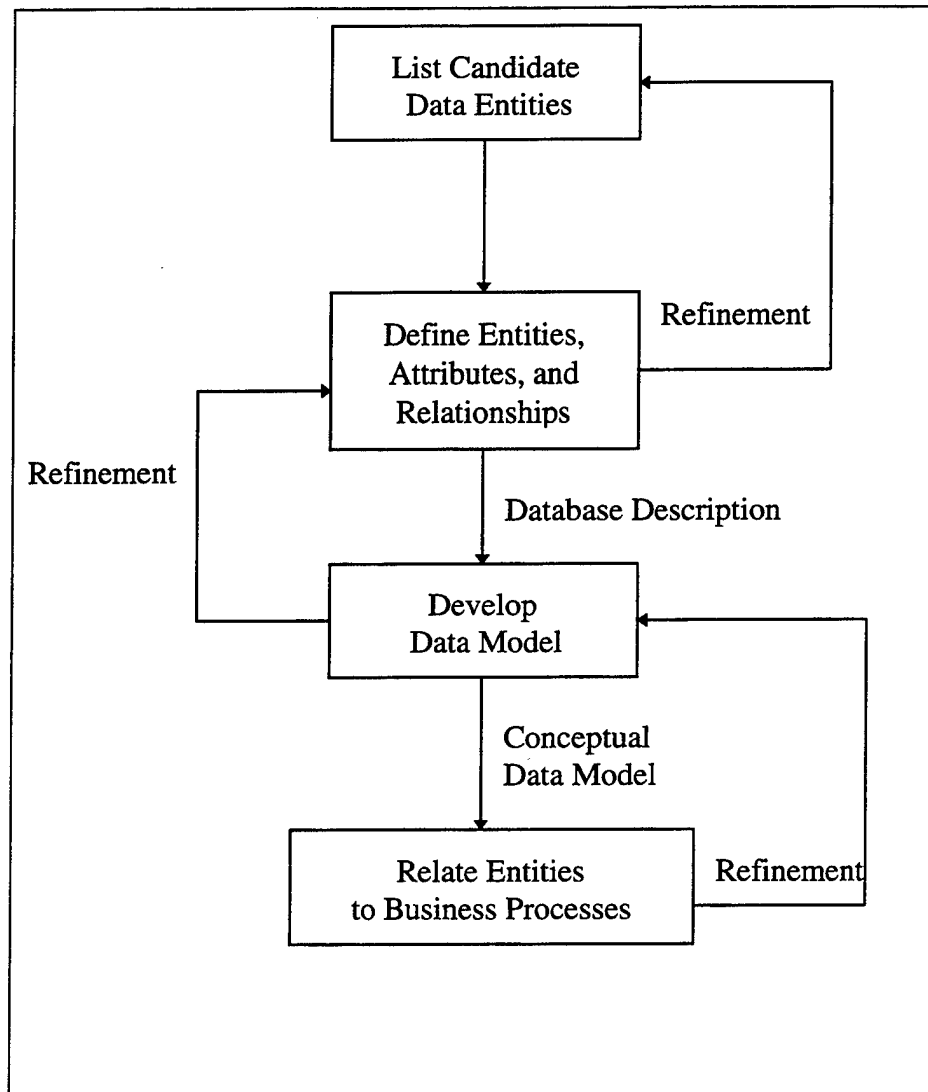
Figure 3-1. Data Model Development Methodology
