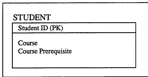
Figure 3-4. Entity in Second Normal Form
