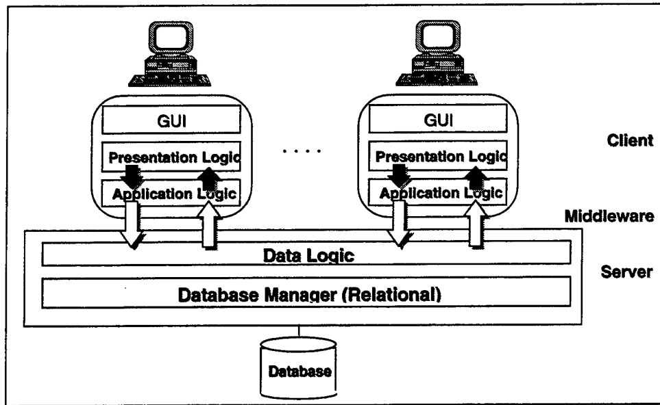
Figure 2-3. Target Client/Server Open Architecture
