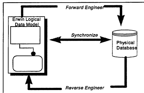
Figure 3-8. ERwin Forward and Reverse Engineering, From Ref. [12]
