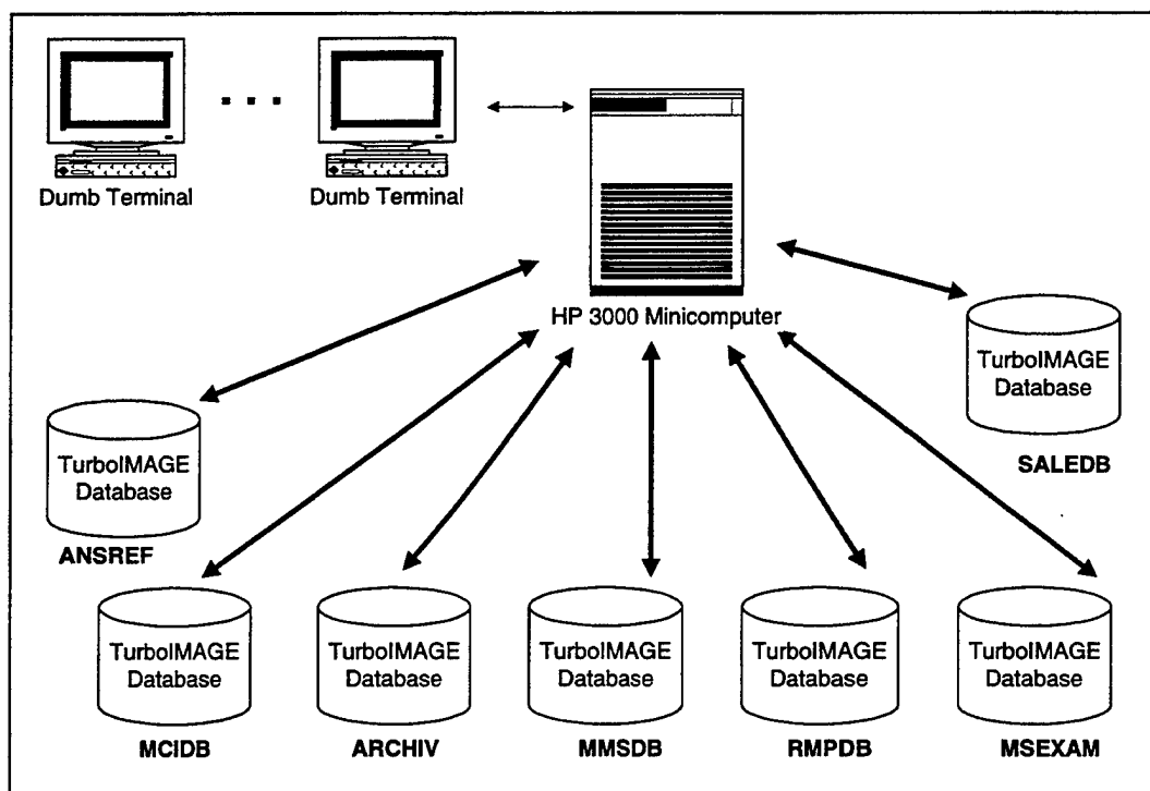
Figure 2-1. MCI AIS Databases
