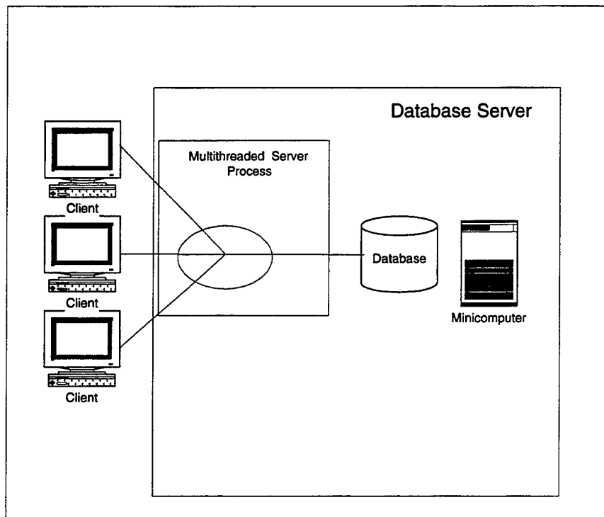
Figure 3-11. Multithreaded Database Server Architecture, After Ref. [5]
