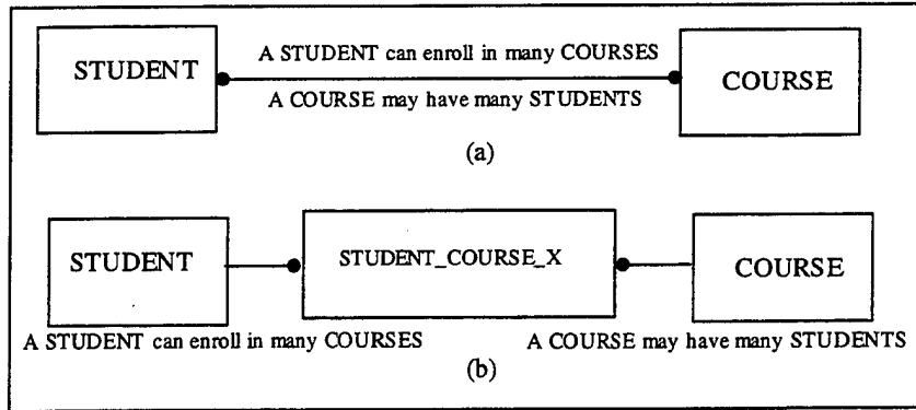
Figure 3-9. Resolved Many - to - Many Relationships
