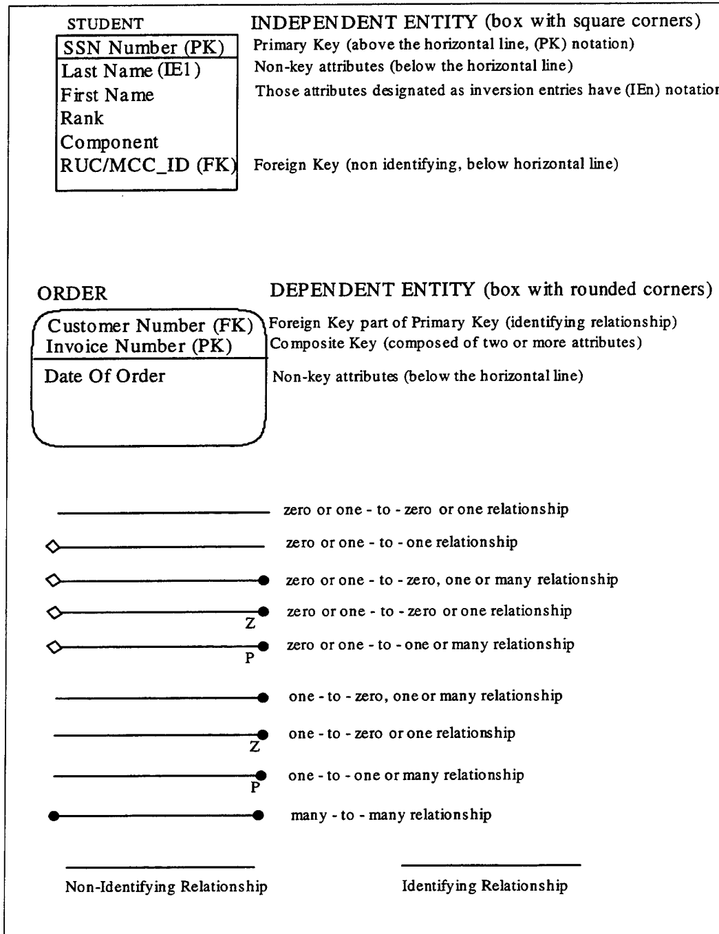
Figure 3-5. Common IDEF1X symbols
