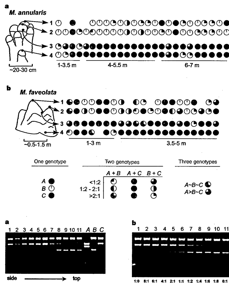
Figure 2 Symbiont zonation in columns of M. annularis . a, b, TaqI digests of srRNA genes. a, Transect from column side to top (lanes 1–11; positions shown in c) and standards for Symbiodinium A, B and C. b, Standards (see Methods). Lane 1, C alone; 2–10, B + C mixtures (numbers below are C:B ratios); 11, B alone. c, Column sampled in a; symbols 1–11 (dark, Symbiodinium C; white, Symbiodinium B) represent the data in lanes 1–11, respectively in a. d, Zonation in 14 columns from 14 colonies sampled as in c (differences in shading are for clarity only); x-axis, location relative to lower side and top centre; y-axis, genotype ranging from all C to all B or all A (A in one column only); z-axis, depth. e, Zonation in a column transplanted to 90° from vertical for 6 months, presented as in c. f, Zonation in 7 columns (all at a depth of 6 m) transplanted and sampled along two transects (white and black) as in e, presented as in d; zonation in natural columns at a depth of 6 m (from d) are plotted for comparison (grey).
