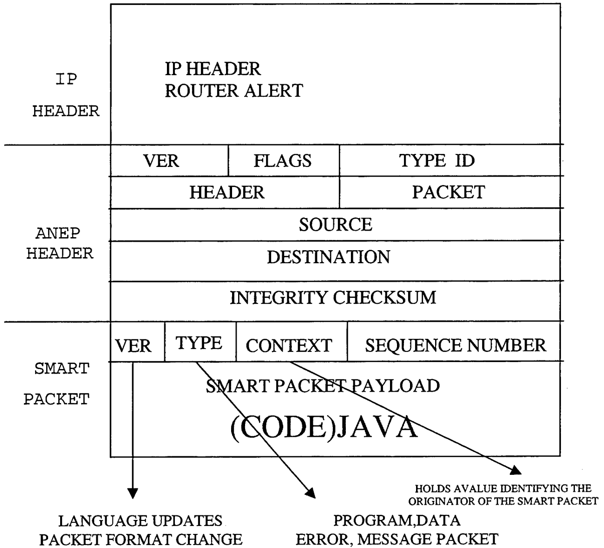
Figure 3.13 Smart Packet Format.
