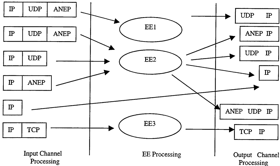
Figure 2.5. Active Node Processing.
