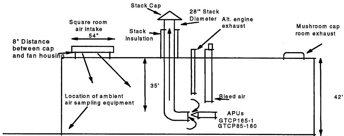
Figure 2-7 APU Test Facility Kelly AFB
