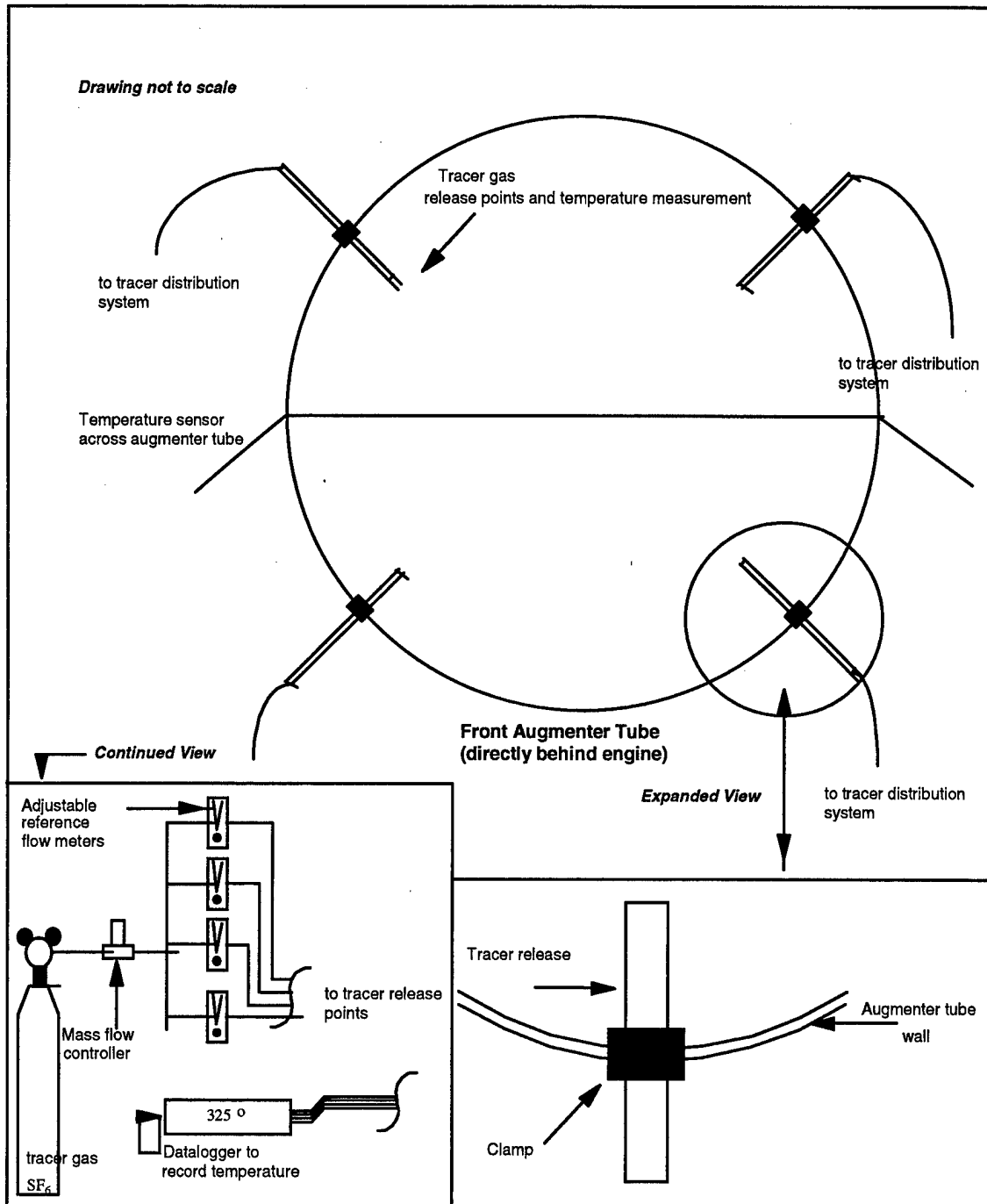
Figure 2-16 Tracer gas distribution system for the augmenter tube at Laughlin AFB
