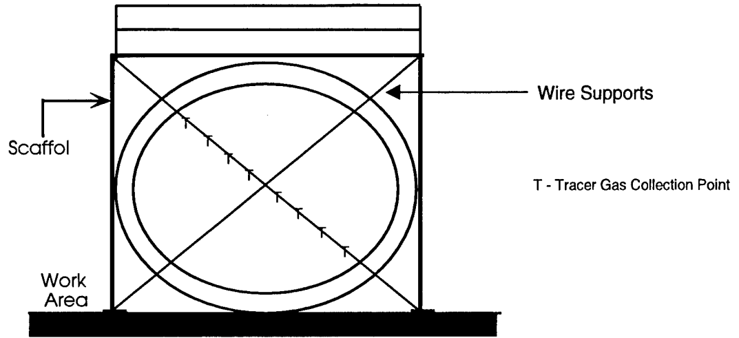
Figure 2-40. Barnes Air National Guard Base Tracer Collection Points
