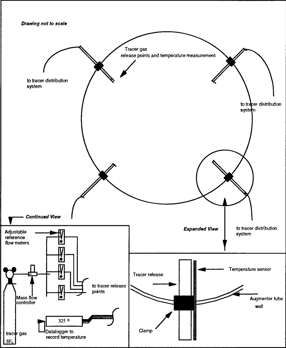
Figure 2-30 Tracer gas distribution system for an augments tube
