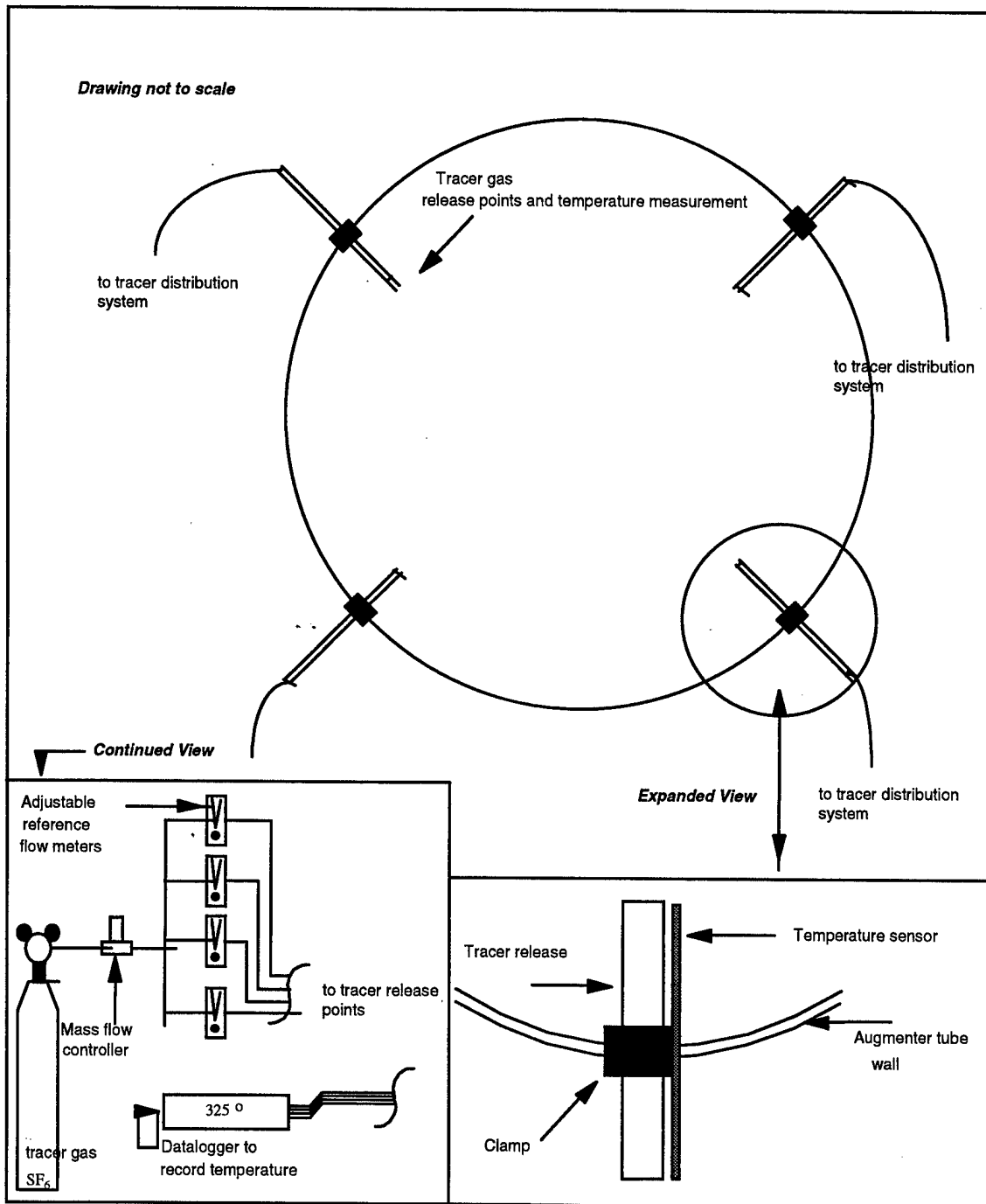
Figure 2-39. Tracer gas distribution system for an augmeter tube
