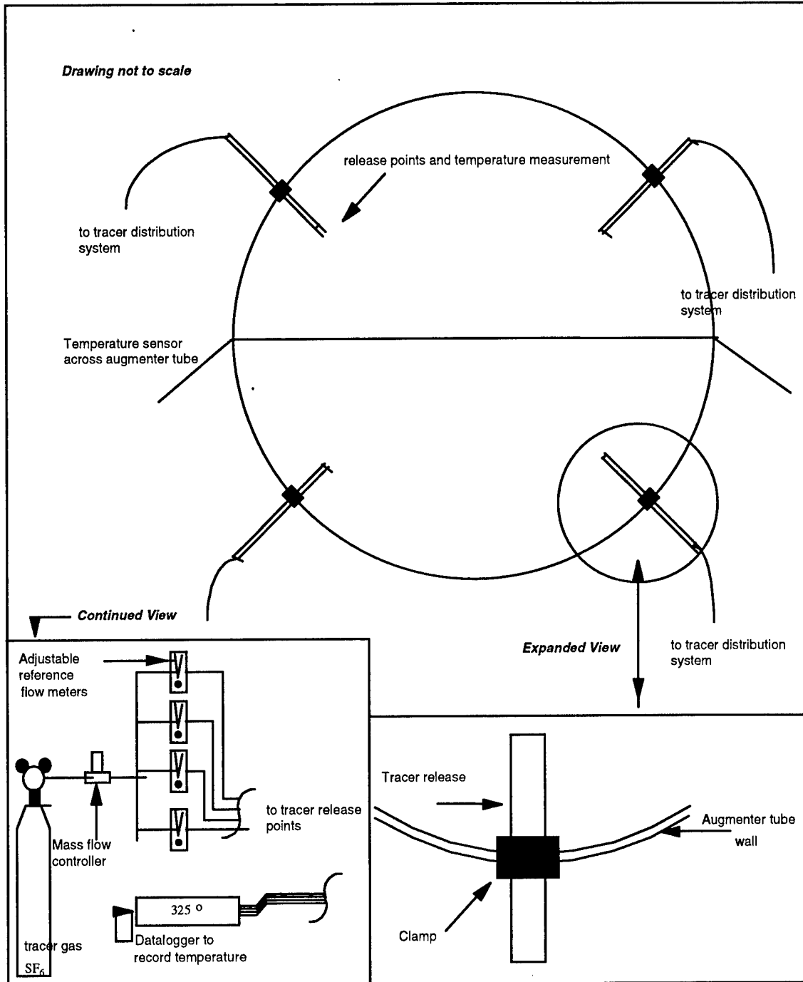
Figure 2-5 Tracer gas distribution system for the augmenter tube
