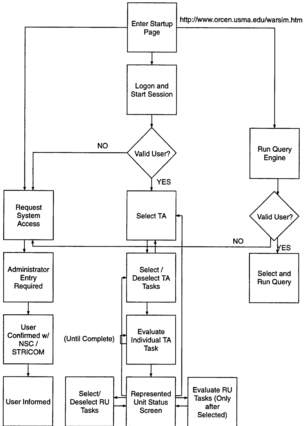
Figure 7. User Navigation.
