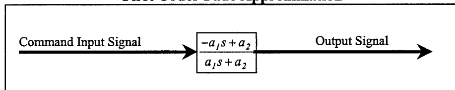
Figure 4-5 Transfer Function Model for the e^{\tau s} Time Delay Using First Order Padé Approximation
