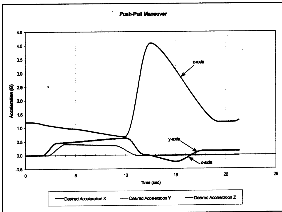
Figure 8-3 Push-Pull Profile
