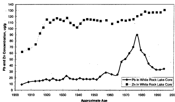
Distribution of sedimentary lead (Pb) and sedimentary zinc (Zn) in a sediment core from White Rock Lake, Dallas, Texas.
