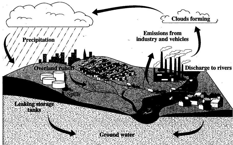
Pathways by which methyl tert-butyl ether moves through the environment.
