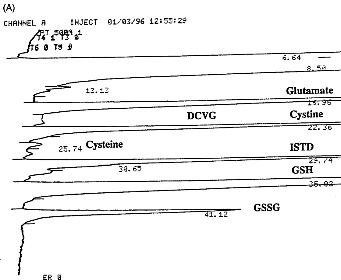
FIGURE 1. Representative HPLC chromatograms of human blood derivatized for detection of DCVG. Blood samples were deproteinated with perchloric acid, treated with bathophenanthroline disulfonate as an antioxidant and with L- \gamma -glutamyl-L-glutamate as an internal standard (ISTD), and acid extracts were derivatized with iodoacetic acid and 1-fluoro-2,4-dinitrobenzene as described in Materials and Methods. N -Dinitrophenyl derivatives of glutamate, DCVG and the ISTD, N,N -bis-dinitrophenyl derivatives of cystine and GSSG, and S -carboxymethyl- N -dinitrophenyl derivatives of cysteine and GSH were separated on an amine column by gradient HPLC using a methanol-acetate solvent system. Derivatives were detected by absorbance at 365 nm and were quantitated by integration with respect to derivatives of authentic standards. (A) HPLC chromatogram of blood from one individual at time 0 before Tri exposure. It is important to note that retention times will vary and decrease with use of the column because of derivatization of amine groups on the column by unreacted 1-fluoro-2,4-dinitrobenzene. This is compensated for by adjusting the concentration of acetate in the solvent.
