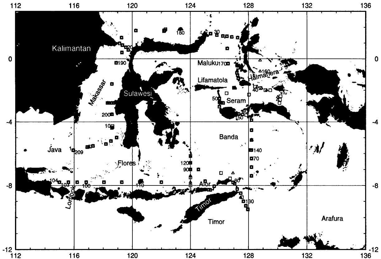
Figure 1. CTD/Hydrographic stations from Phase I ( August-Sep 1993 and Jan-Feb 1994)
