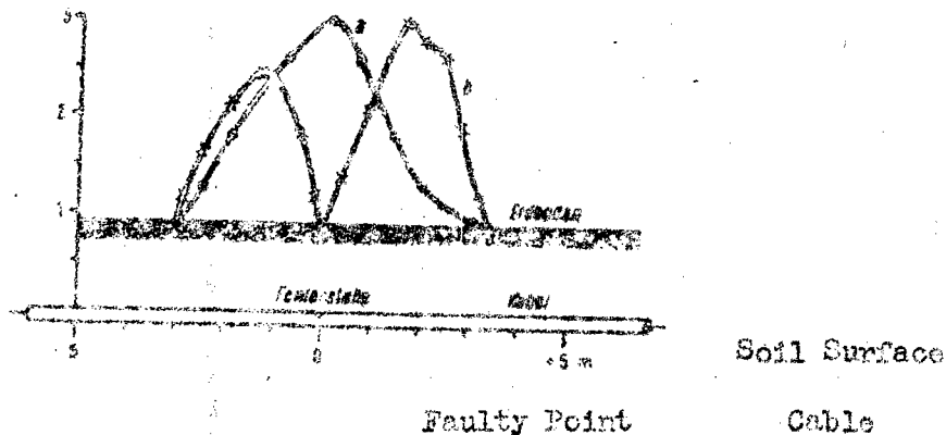
Figure 3. Course of field of the HF-impulse field at the faulty point. Curves a: Coil lined up with cable; Curve b: Coil vertical to the cable.
