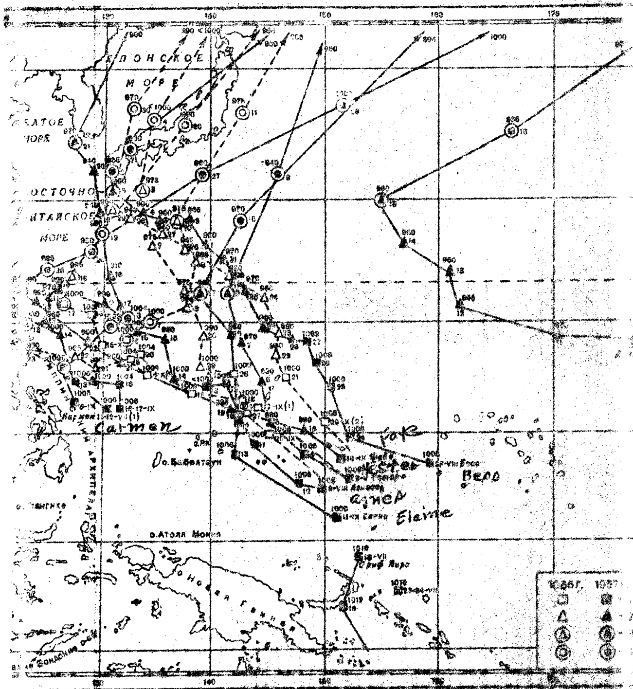
Figure 1. Trajectory of cyclones. Stages of development of typhoons. 1, tropical depression; 2, typhoon; 3, moment of transformation; 4, transformed typhoon. Numbers signify dates and pressure at center.
