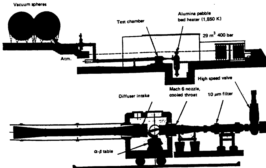
Figure 1. S4MA hypersonic wind tunnel (80403)
