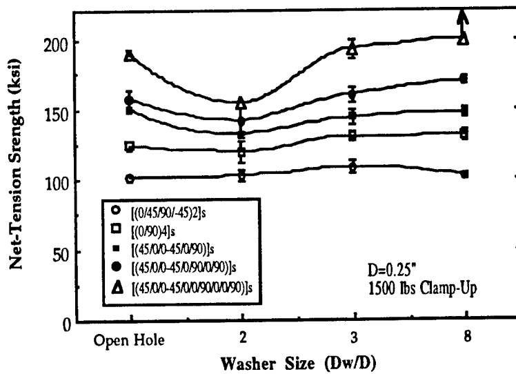
FIGURE 16. EFFECT OF WASHER SIZE ON NOTCH STRENGTH OF FILLED-HOLE LAMINATES (CONSTANT CLAMPING LOAD)
