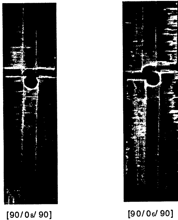
FIGURE 11. RADIOGRAPHS OF DAMAGED [90/0 a /90] AND [90/0 e /90] LAMINATES
