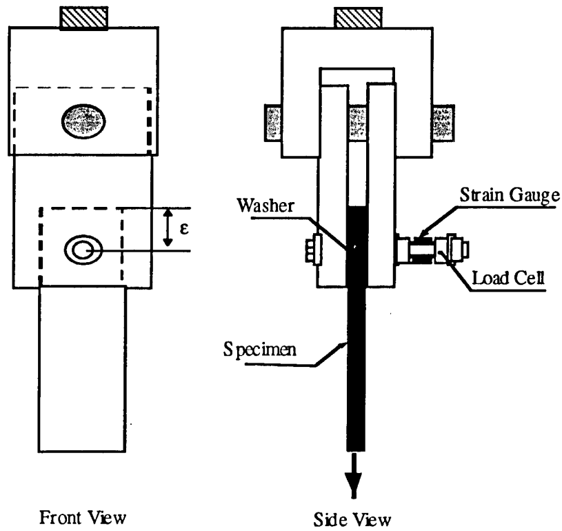
FIGURE 3. GEOMETRIES OF THE BOLTED-JOINT TEST SETUP
