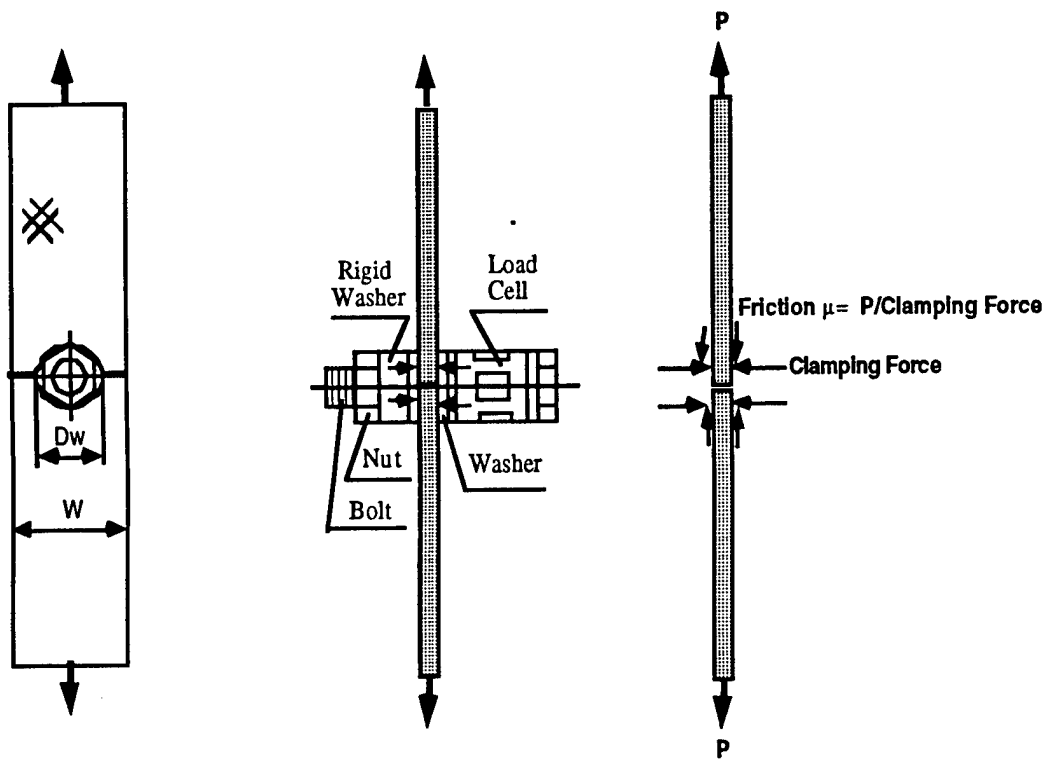
FIGURE 19. SCHEMATIC OF THE TEST SETUP FOR MEASURING FRICTION COEFFICIENT BETWEEN A COMPOSITE PLATE AND A WASHER
