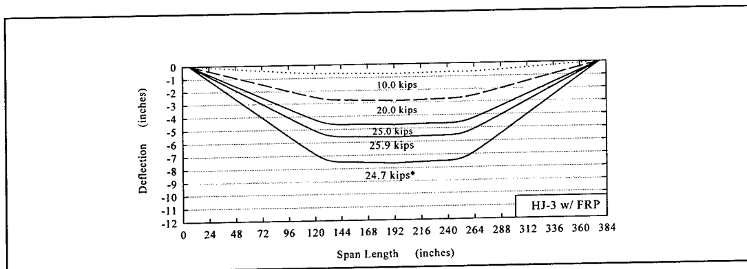
Figure 21. Deflected shape for HJ-3.
