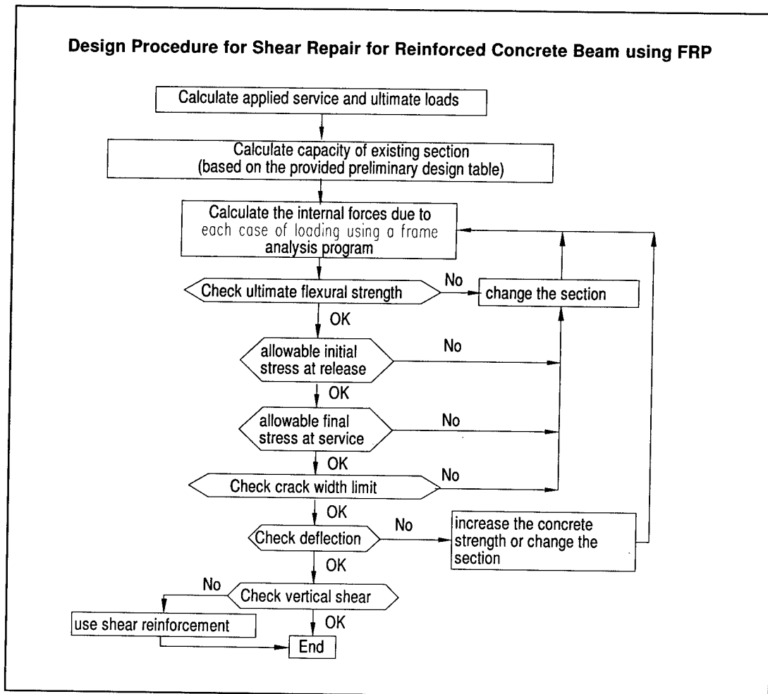
Figure 42. Shear repair design procedure.
