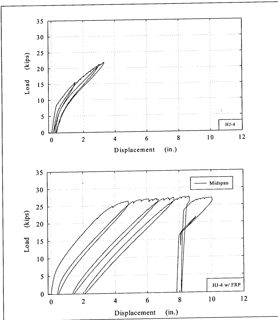
Figure 20. Load versus deflection cycles for HJ-4.
