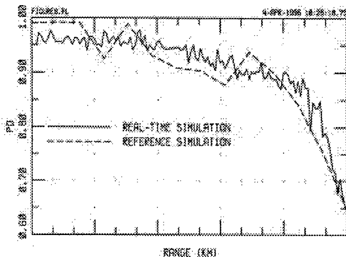
Figure 8. Real-time vs reference simulation
