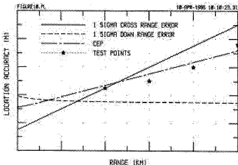
Figure 10. CEP approximation vs range
