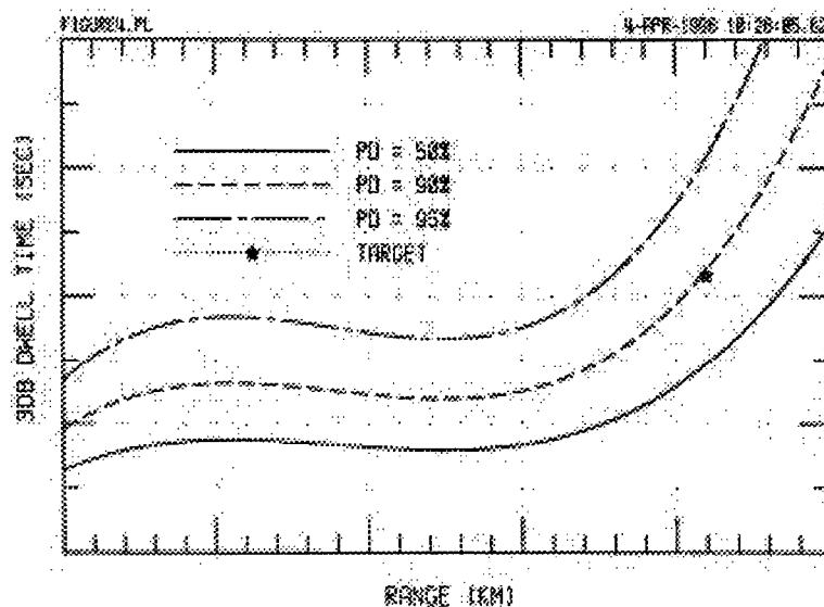
Figure 4. Expand Dwell Time by Range (Scan angle = 0 degrees)
