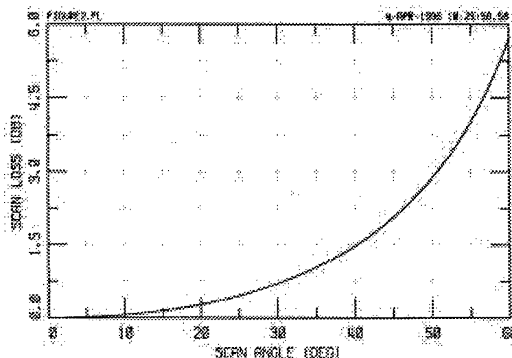
Figure 2. Azimuth Scan Loss
