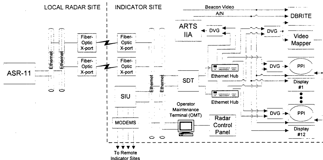
FIGURE 3.3-1. ASR-11 TO ARTS IIA INTERFACE (OPERATIONAL CONFIGURATION)
