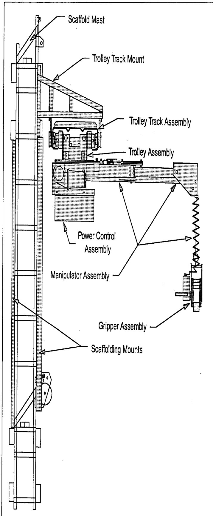
Figure 9. MAMA design.
