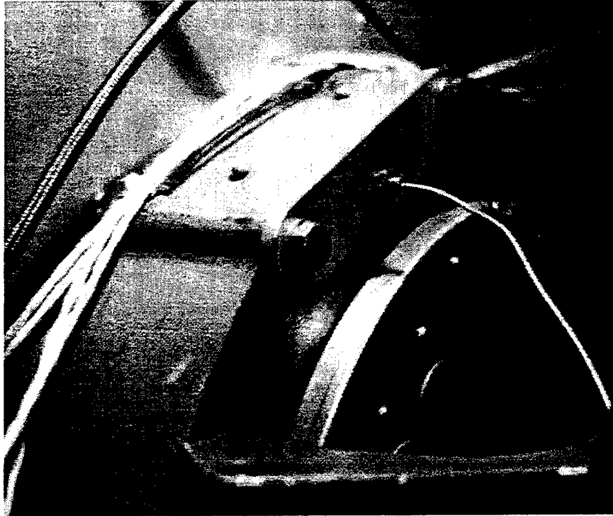
Figure 9. Proximeter mounting
