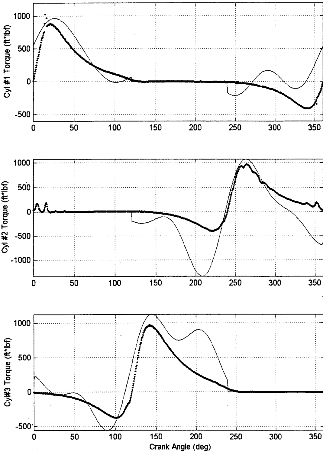
2000 RPM, 160 ft*lb Cylinder Gas Torques
