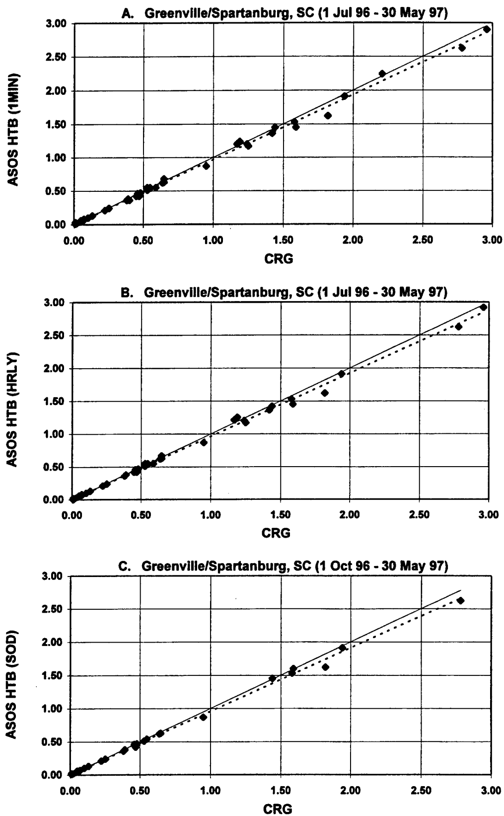
Figure 3.1 ASOS HTB versus CRG (SRG) at GSP for (A) 1MIN, (B) HRLY, and (C) SOD.
