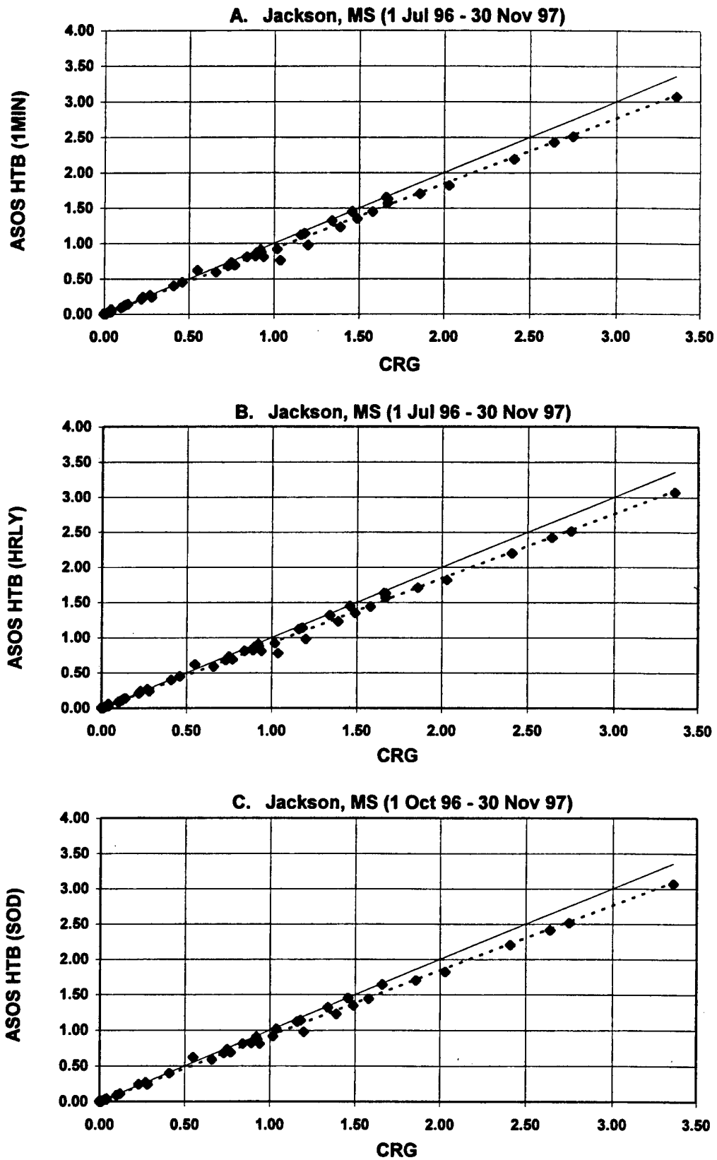
Figure 3.2 ASOS HTB versus CRG (SRG) at JAN for (A) 1MIN, (B) HRLY, and (C) SOD.
