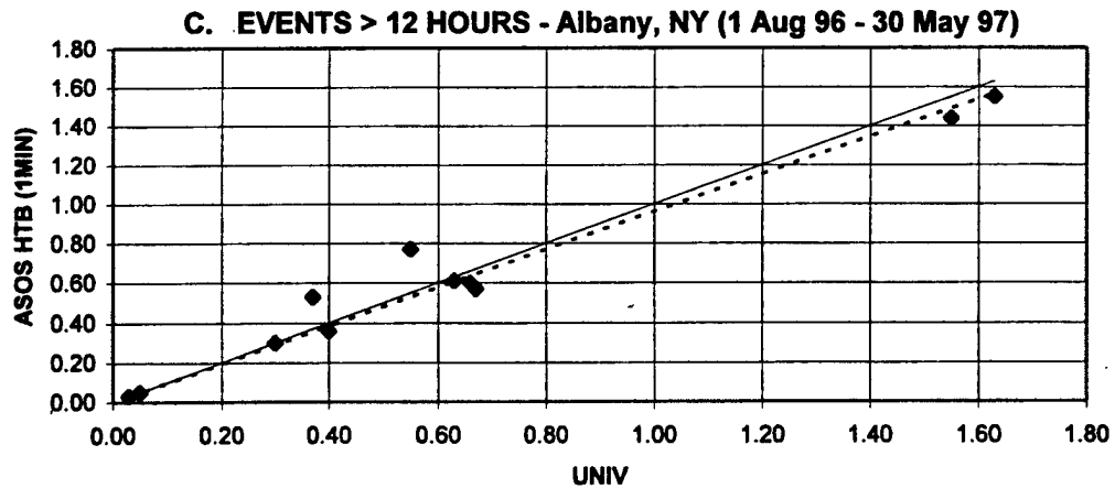
Figure 3.6 ASOS HTB 1MIN versus UNIV at ALB for (A) All Events, (B) Events < 12 Hours, and (C) Events > 12 Hours.
