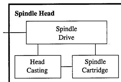
Figure 3.5. Additional decomposition for spindle head
