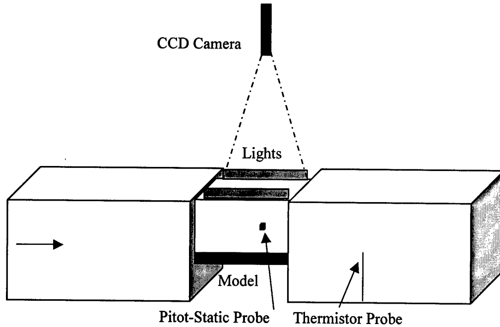
Figure 5 Experimental Setup
