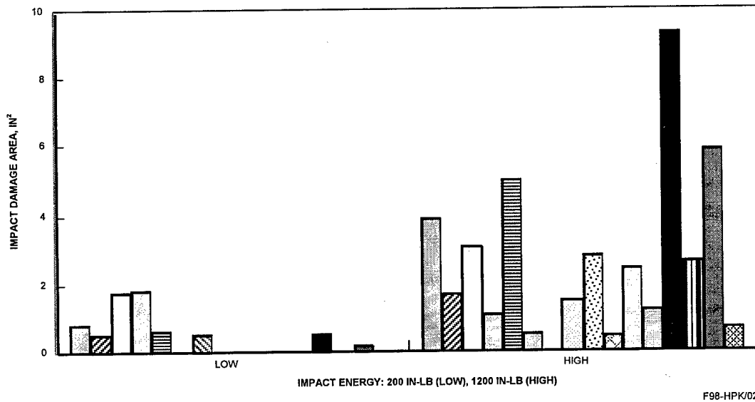
FIGURE 2. EFFECTS OF IMPACT ENERGY ON DAMAGE AREA, RANK 1/14
