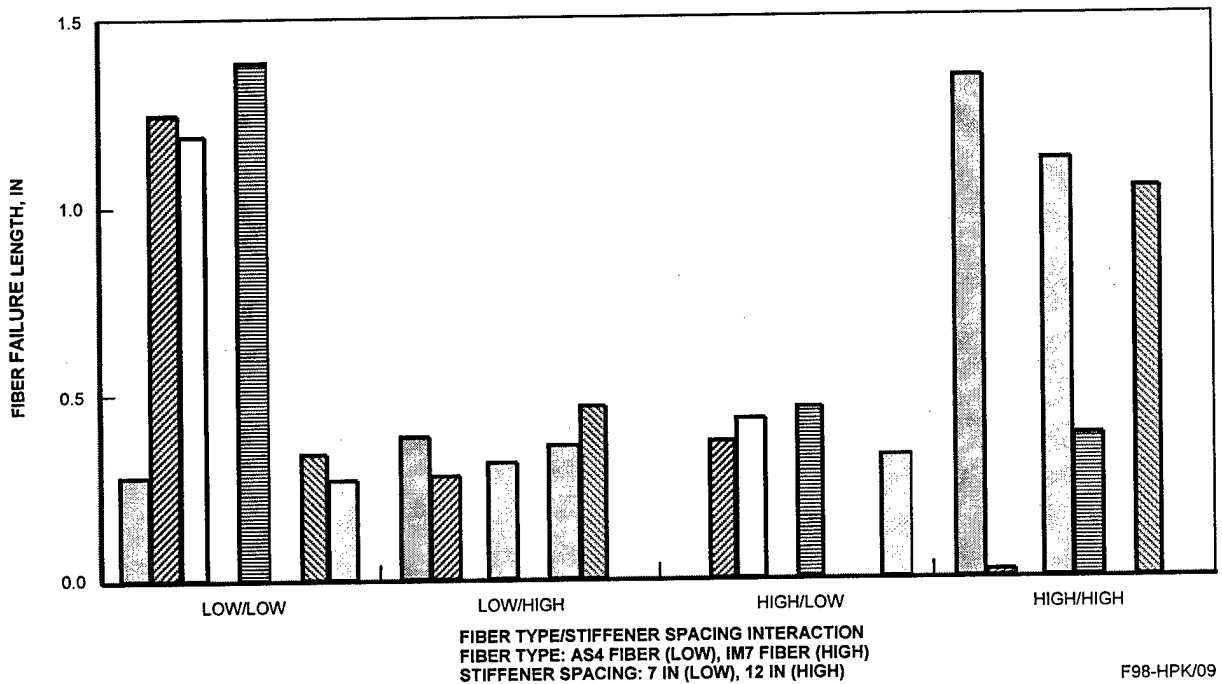
FIGURE 9. FIBER TYPE/STIFFENER SPACING INTERACTION ON FIBER FAILURE LENGTH
