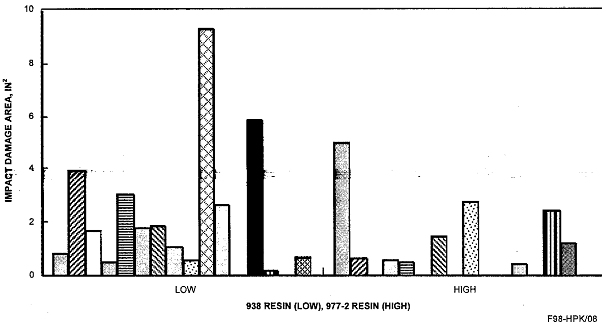
FIGURE 8. EFFECTS OF MATRIX TYPE ON IMPACT AREA, RANK 3/14
