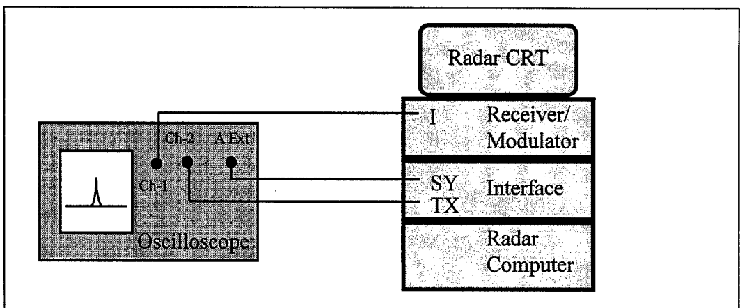
Figure 5. Radar signal analysis test hardware configuration.
