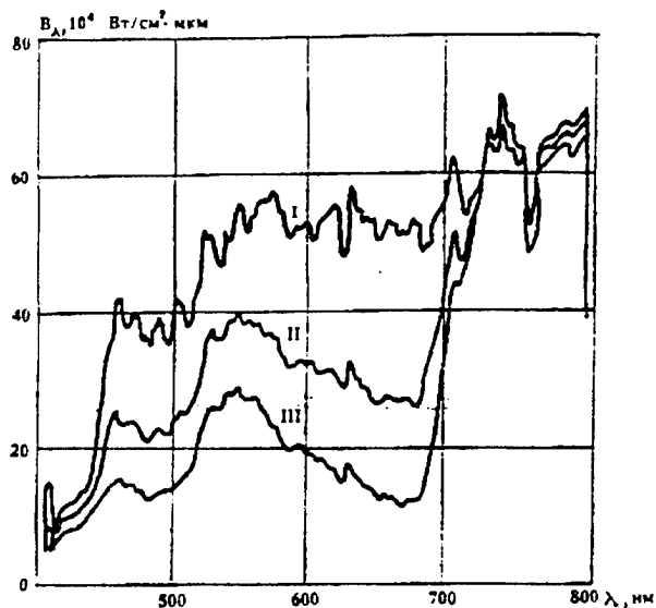
Average values of spectral brightness of various geosystems on test sector: typical American prairie (I), forest (II), and bare soil with areas of dry vegetation (III). x-axis: \lambda , nm; y-axis: Wave_{\lambda} , 10^4 W/cm^2 \times \mu m .
