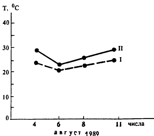
Surface radiation temperatures of the prairie (I) and forest (II) measured by the Mara radiometer during the experiment, August 1989.
