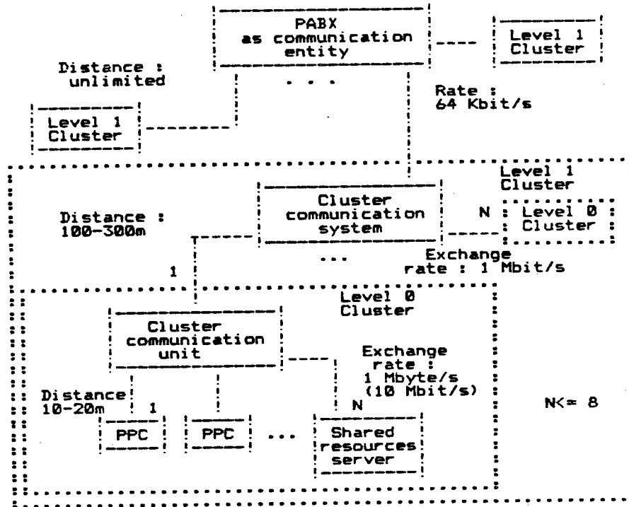
Figure 1. "Lencluster" LAN
