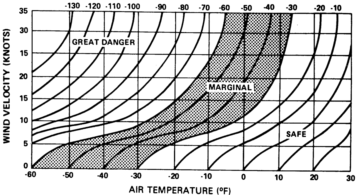
Figure 4-2. Wind Chill Graph - Equivalent Temperature Curves
