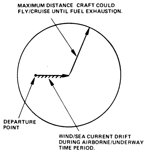
Figure 5-2. Maximum Area of Possibility
