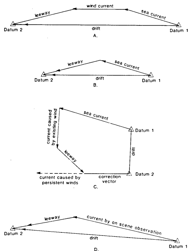
Figure 5-3. Vector Plots of Surface Drift Forces
