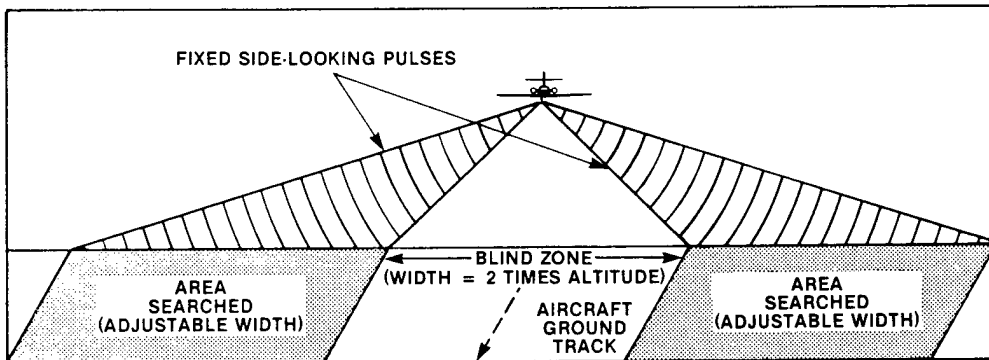
Figure 6-15. Side-Looking Airborne Radar (SLAR)
