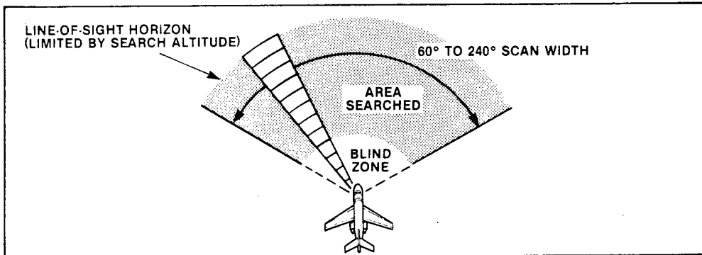
Figure 6-14. Forward-Looking Airborne Radar (FLAR)
