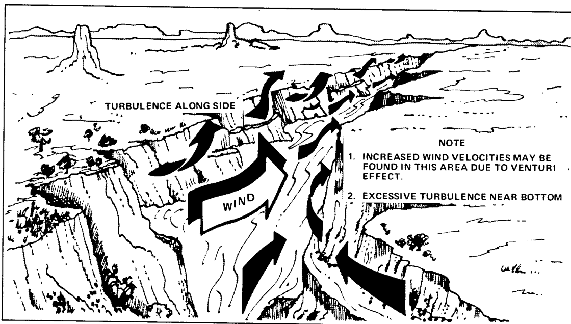
Figure 8-2. Wind Flow in Valley or Canyon
