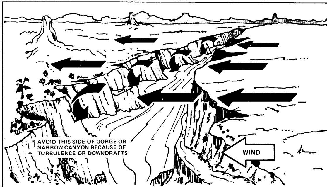
Figure 8-1. Wind Flow Over Gorge or Canyon
