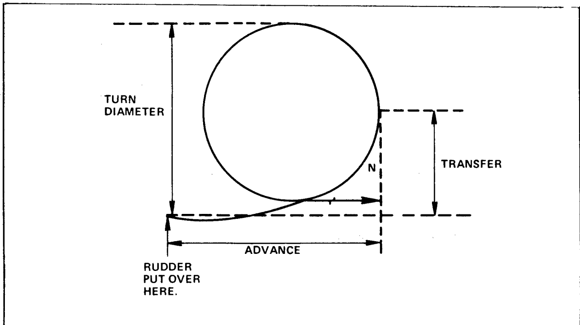
Figure 6-7. Typical Vessel-Turning Circle
