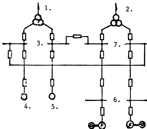
Figure 2. 6 kV Plant-Used Electrical Connections
