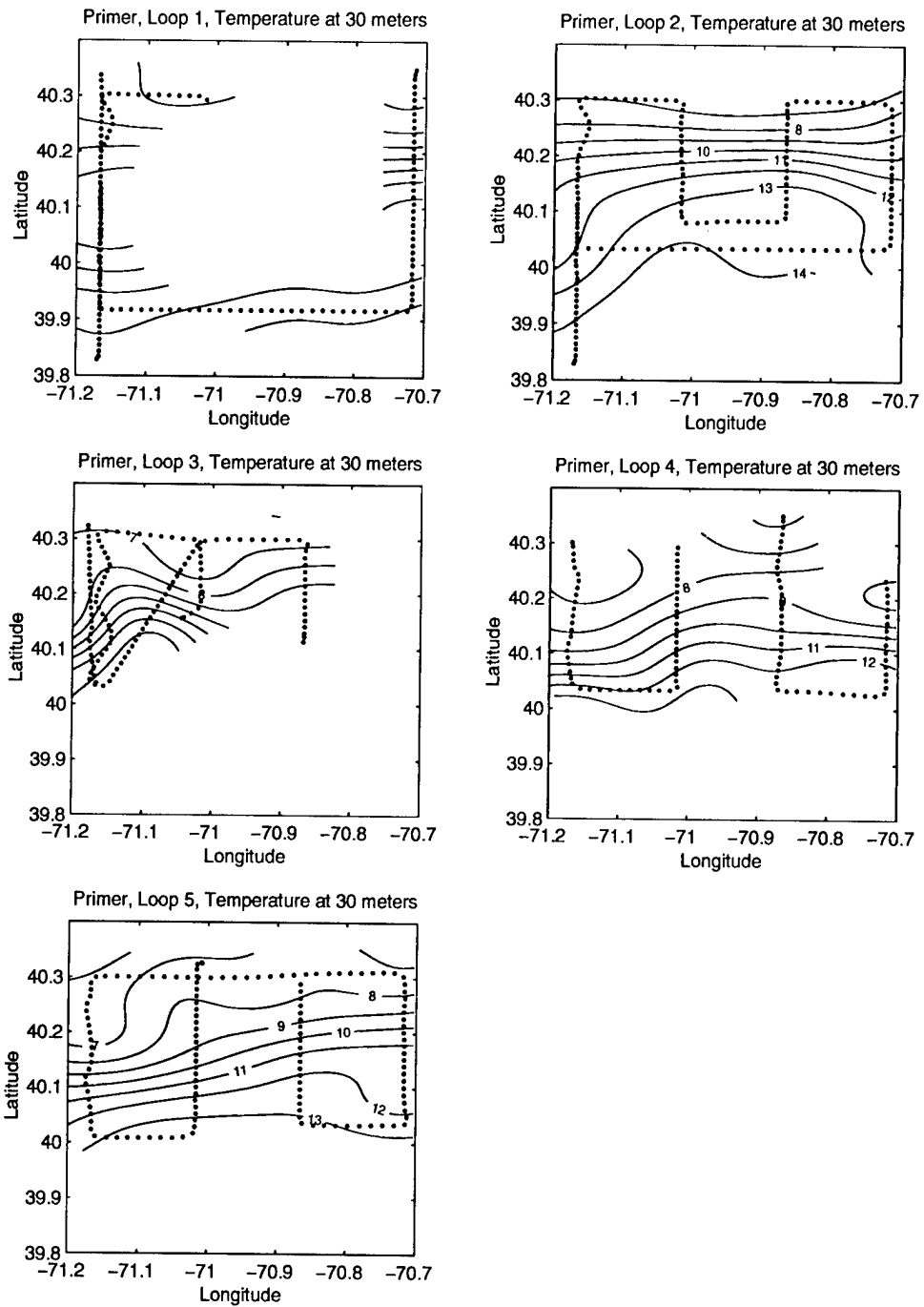
FIGURE 7. Seasor grids with temperature contours for 30 meter depth.
