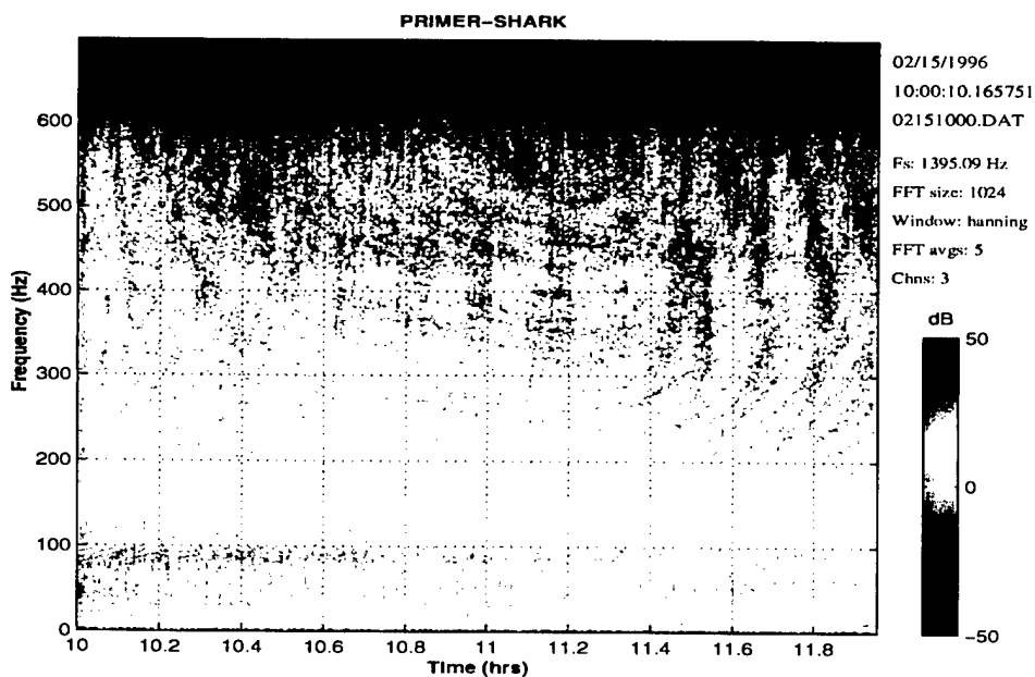
FIGURE 60. Frequency receptions for the Shark just before recovery. The circular patterns are ship noise frequencies.
