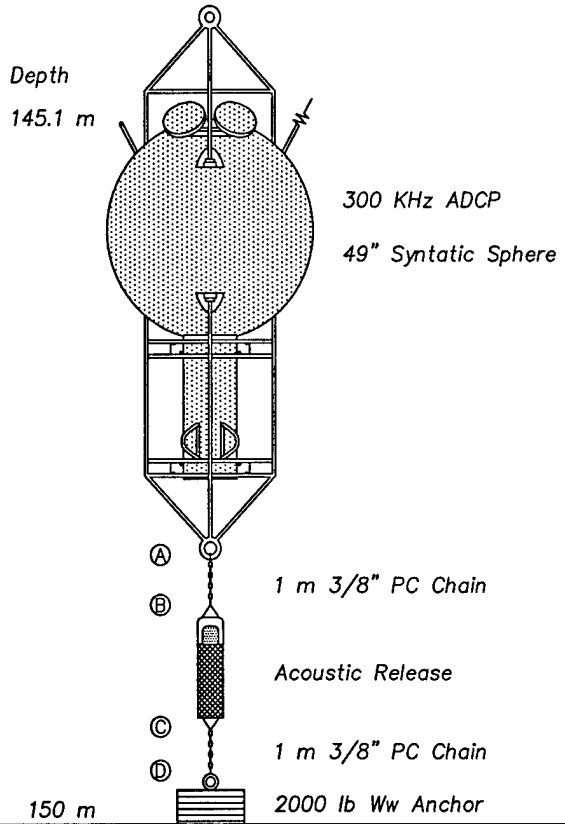
Winter Primer Experiment, 300 KHz ADCP Mooring
