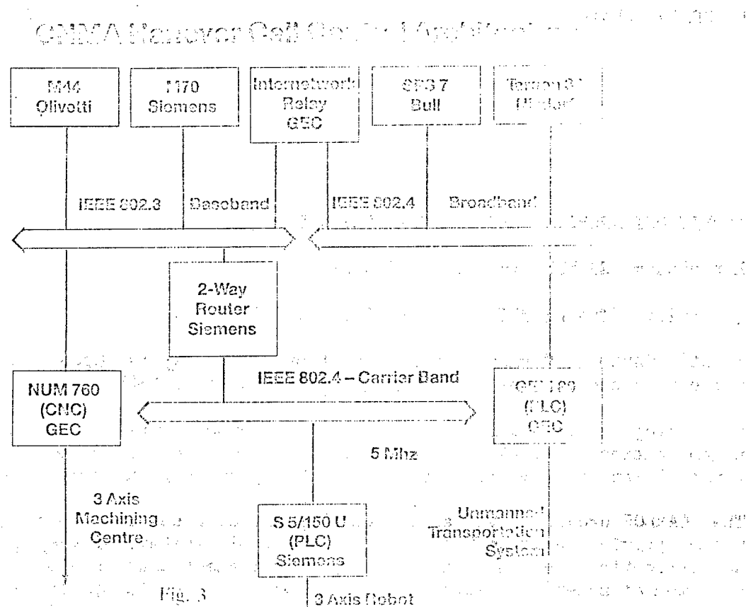
Figure 3 shows the control architecture demonstrated at Hannover.
