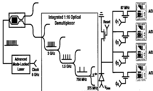
Figure 13. Architecture of a wideband converter. The bandwidth of the sampled signal is reduced in the optical demultiplexor until further processing can be done in the electrical domain.
