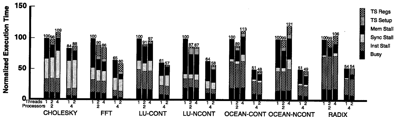
Figure 2: Performance of the baseline software-controlled multithreading scheme.
