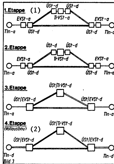
Fig. 3. Possible variants of the construction stages of a digital communications network: — analog transmission path (a); = digital transmission path (d); Tln--subscriber; EVSt--terminal exchange location; TrVSt--transit exchange location; ÜSt--transfer location.
