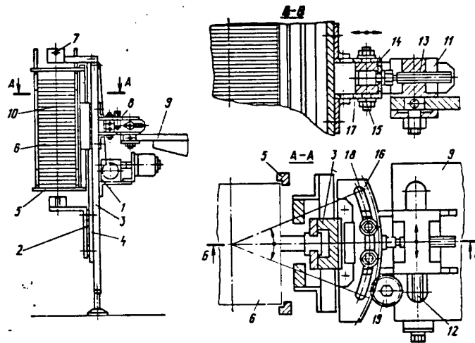
Fig. 2. Billet dispenser.
