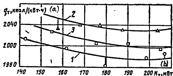
Figure 2. Specific heat consumption in electric power generation:
