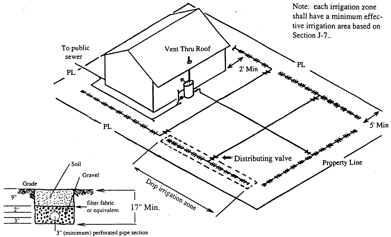
Figure 5—Graywater System Irrigation Layout (conceptual)
