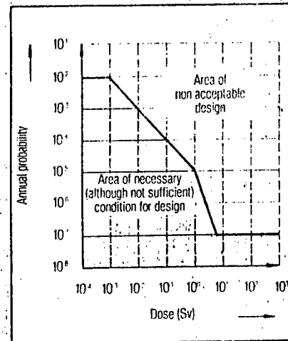
Fig. 8. Limit criterion curve.
