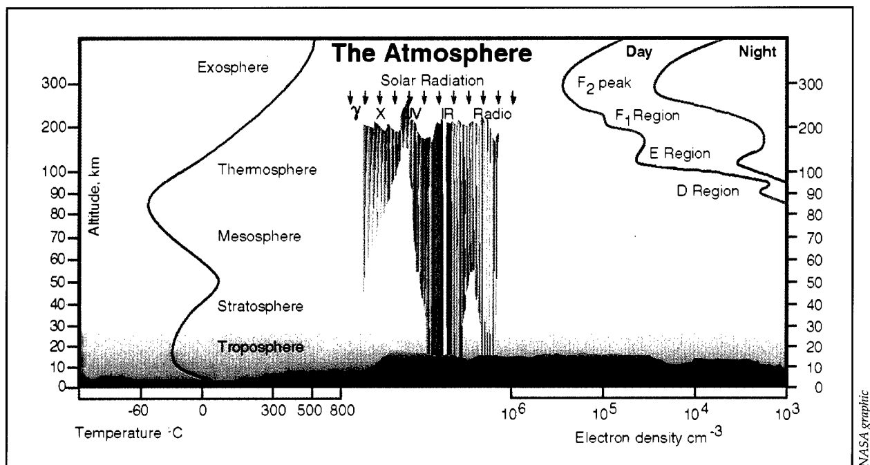
Schematic representation of the atmosphere and the ionosphere. The altitude dependence of the temperature and electron density are shown on the left and right sides, respectively. The spectrum of solar radiation and its atmospheric absorption are shown in the middle. The ionosphere starts at about 70 km. Communication paths between the ground and satellites have to cross the ionosphere and the atmosphere.
