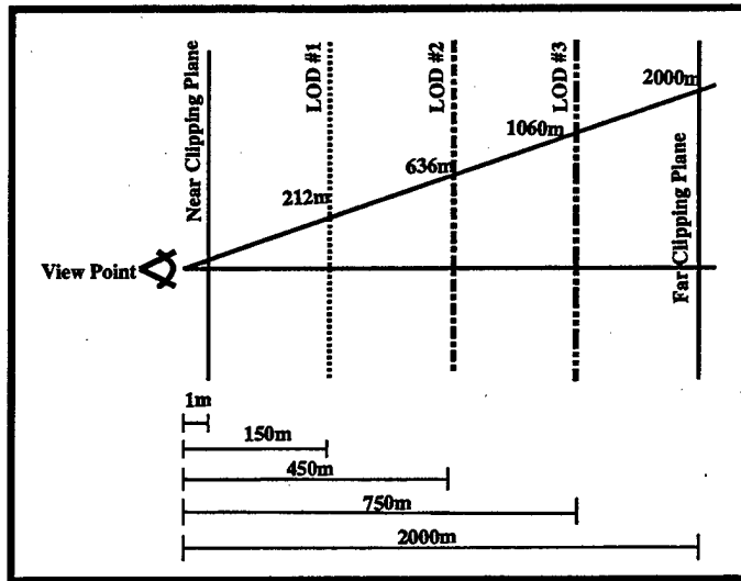
Figure 3.2. LOD Distances
