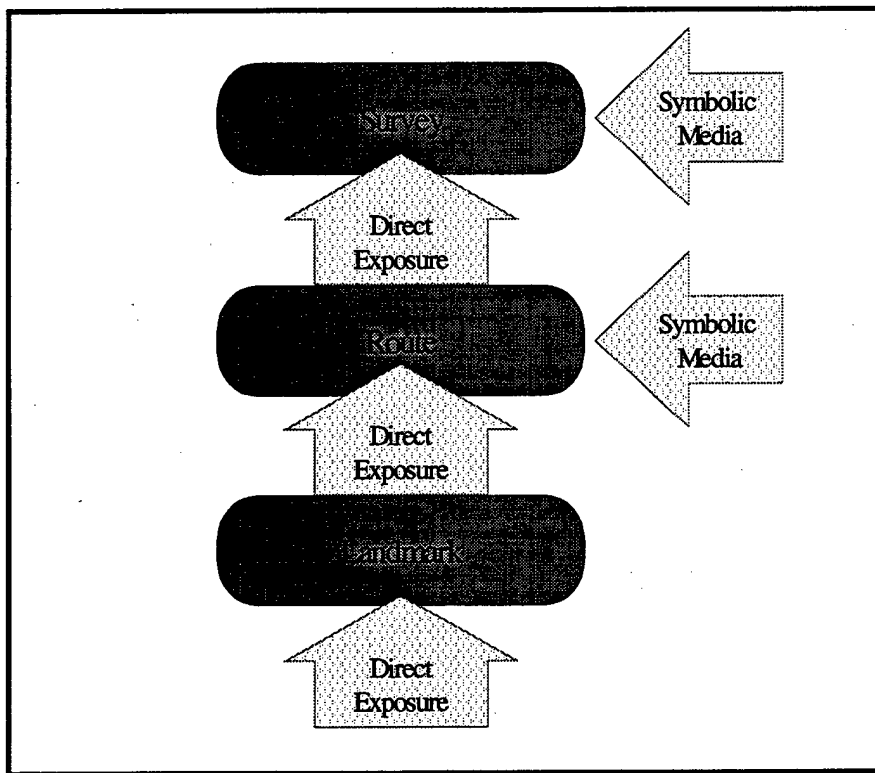
Figure 2.1. Navigation Knowledge.
