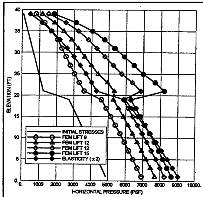
Figure 29. Ramp surface (S1), 4V on 8H slope, sand-H surcharge on layered sand-H over clay base (1 ft = 0.305 m; 1 lbf/ft 2 = 47.9 Pa)
