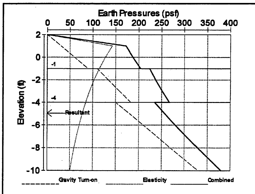
Figure 81. Example 3, levee section, granular soil, irregular ground surface (1 ft = 0.305 m; 1 lbf/ft 2 = 47.8 Pa)
