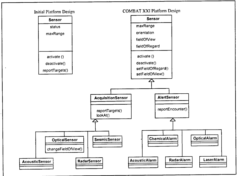
Figure 10. Combat XXI Sensor Component Design.
