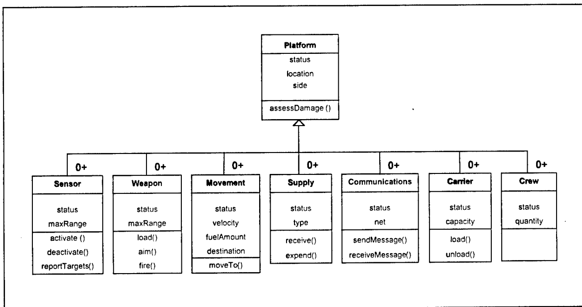
Figure 1. Initial Platform Object Design.
