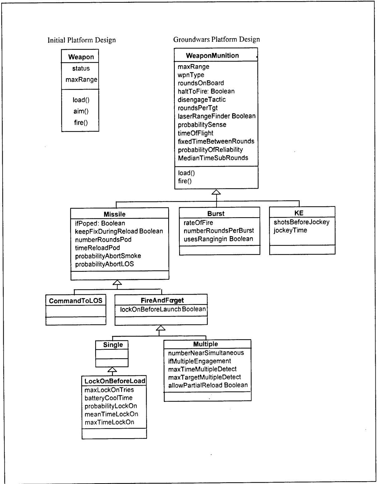
Figure 3. Groundwars Weapon Component Design.
