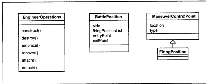
Figure 17. Combat XXI Additional Model Components.
