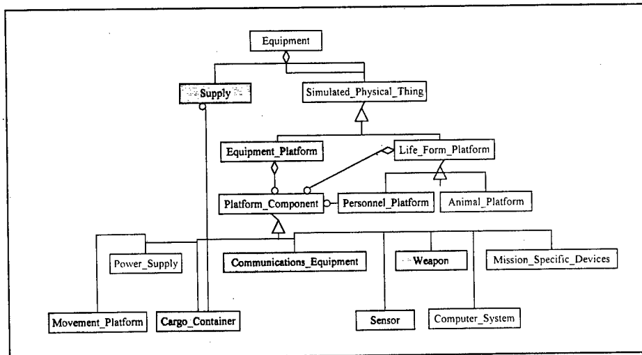
Figure 19. WARSIM 2000 Platform Object Design.
