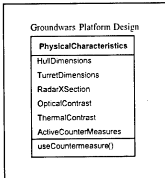
Figure 7. Groundwars Physical Characteristics Component Design.
