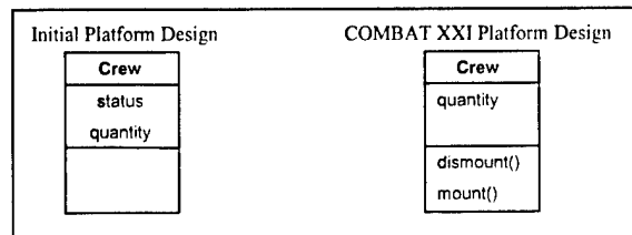
Figure 15. Combat XXI Crew Component Design.
