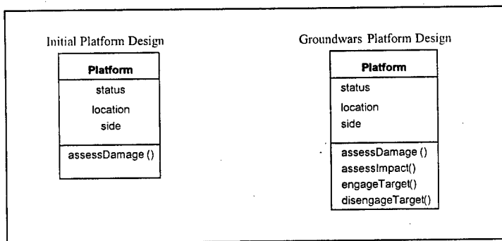
Figure 2. Groundwars Platform Class Design.
