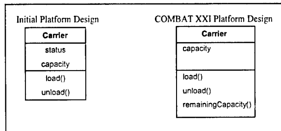
Figure 14. Combat XXI Carrier Component Design.
