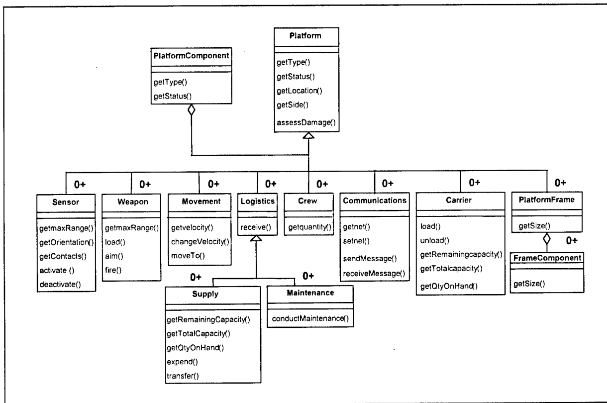
Figure 20. OMSC Final Platform Object Design.
