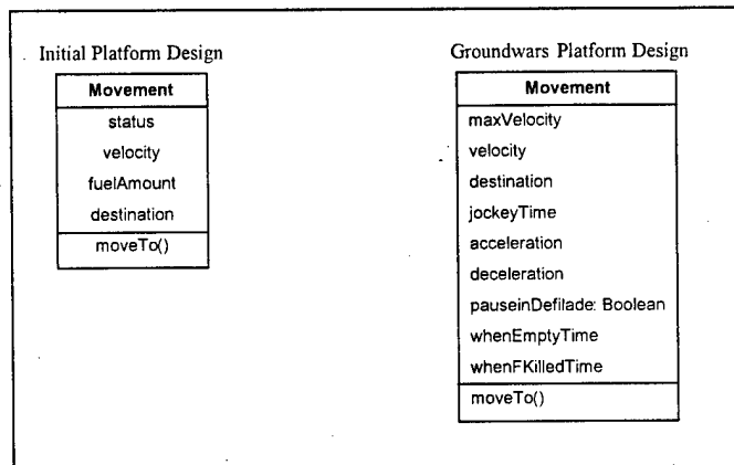
Figure 6. Groundwars Movement Component Design.
