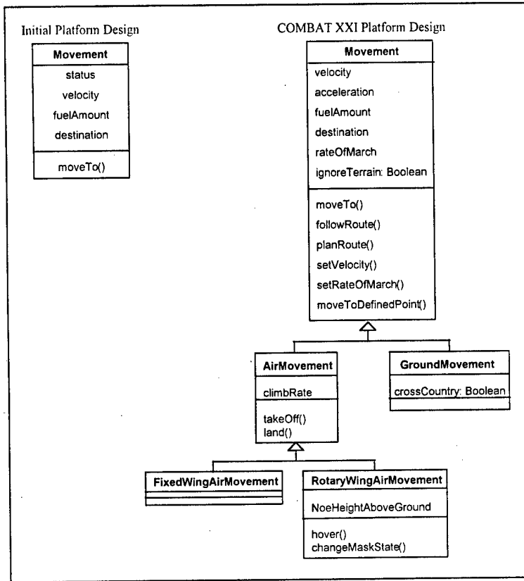
Figure 11. Combat XXI Movement Component Design.
