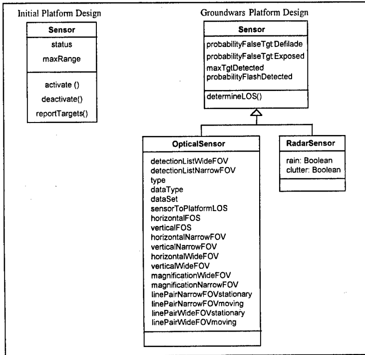
Figure 4. Groundwars Sensor Component Design.
