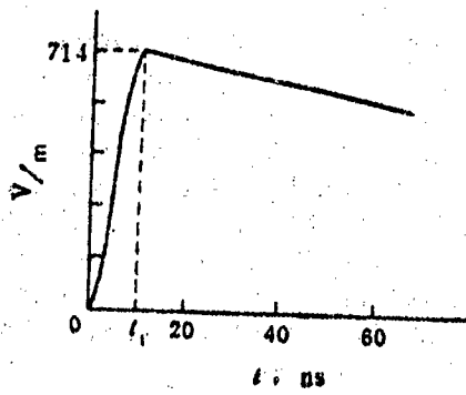
Figure 2. Plane Wave Excitation Waveform
