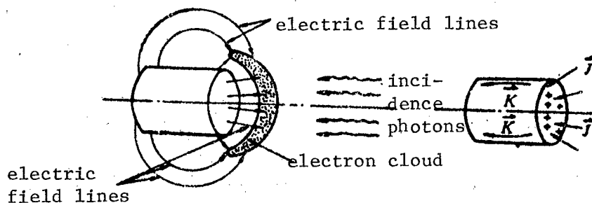
Figure 1. Concept of Cylindrical Test SGEMP Excitation Left: Cylindrical shape and electric field structure Right: J , K and surface charge density (marked by +)
