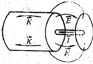
Figure 6. External Shape of Combined Hardwire and Capacitor Excitation
