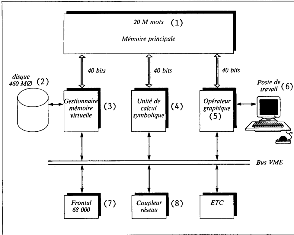
Graph. MAIA System Architecture
