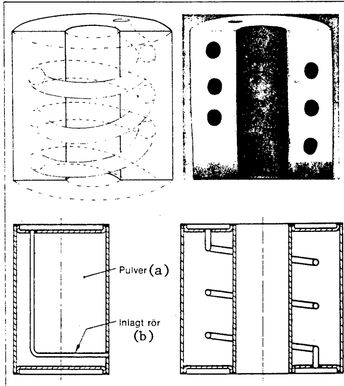
Figure. With powder technology it is possible to create products in almost completed form and to insert channels, for example, into the molded product.
