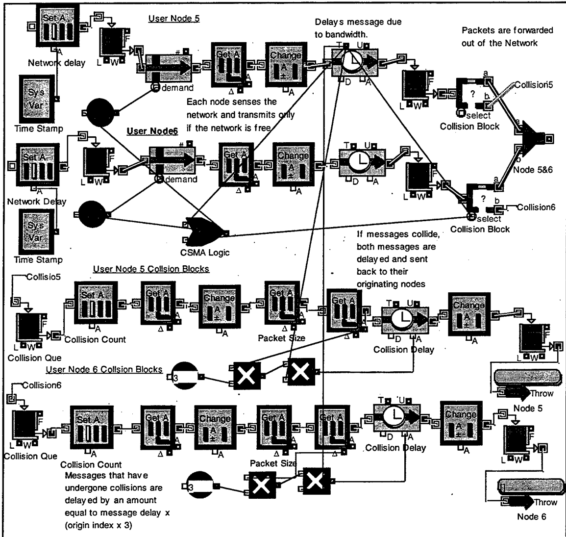
Figure C.6. Second Layer of The Extend 802.11 Wireless Network Layer, Users Five and Six
