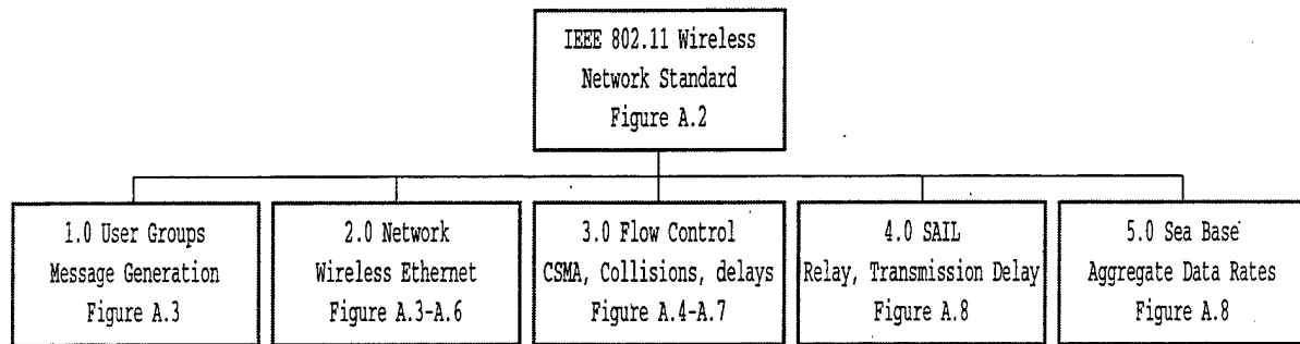
Figure C.1. Decomposition Diagram.
