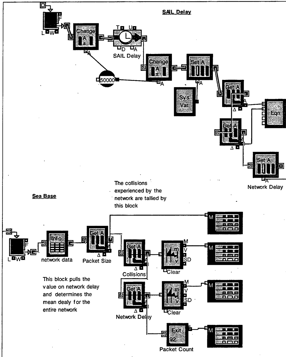
Figure C.8. SAIL and Sea Base Second Layer Blocks.
