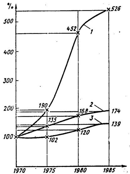
Dynamics of the Volumes of Part Heat Treatment in Coal Machine Building: 1--Heat-treated parts; 2--parts heat-treated in protective atmospheres; 3--chemicothermal treatment
